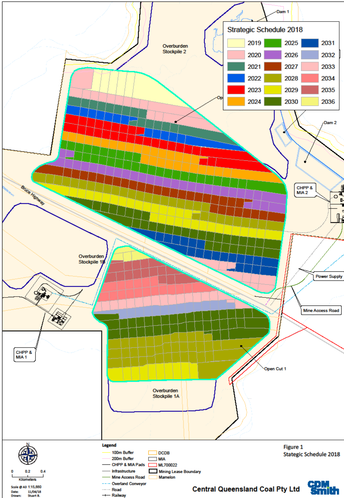
Figure 2-2: Strategic Schedule 2018 [CDM Smith, 2018]
