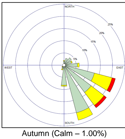
Figure 4-1: Site-Specific Wind Roses by Season for 2014
