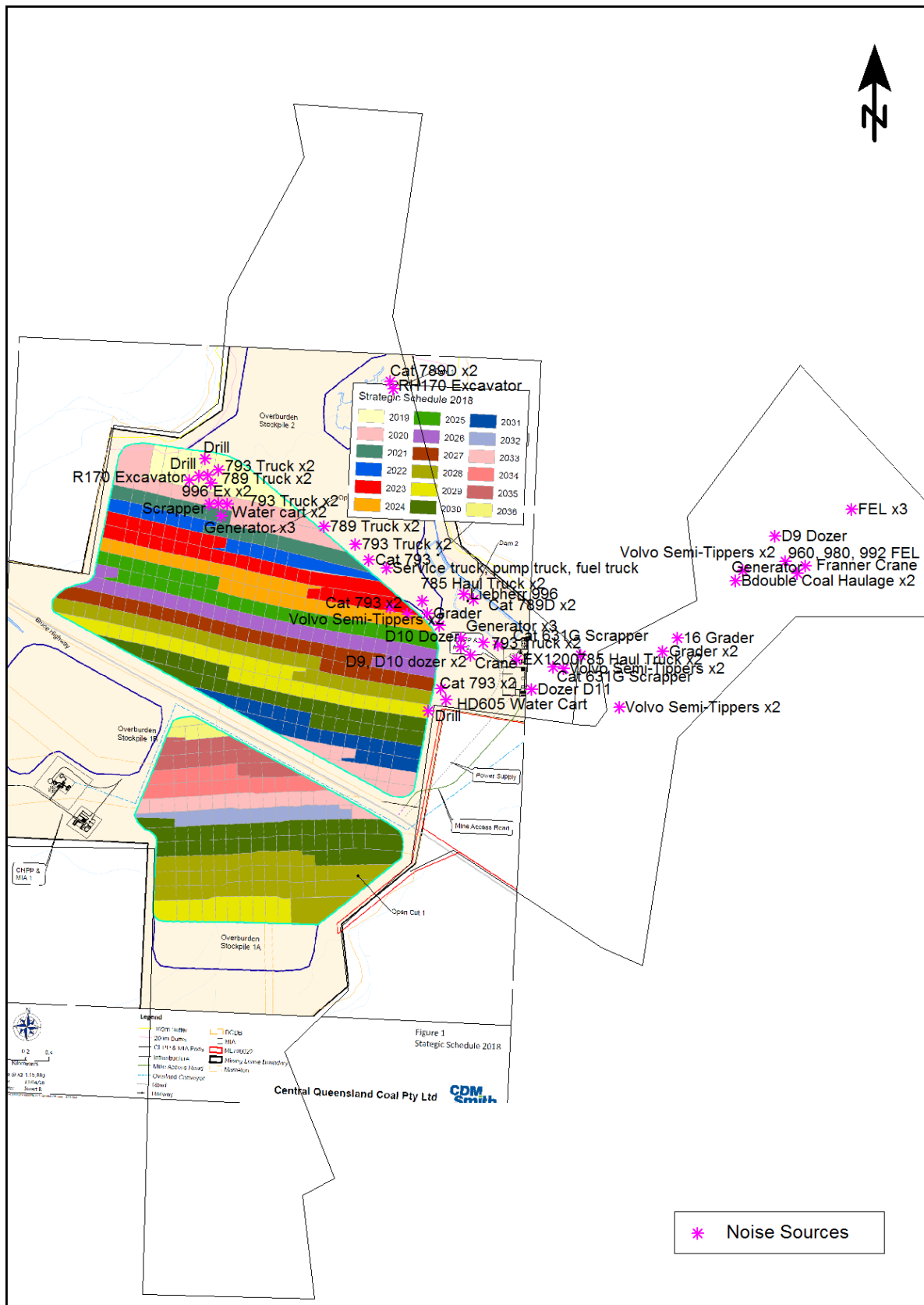
Figure 6-1: Location of Noise Sources as Modelled for Year 3
